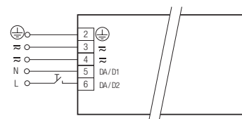
switchDIM PCA T8 EXCEL one4all Ip xtec
